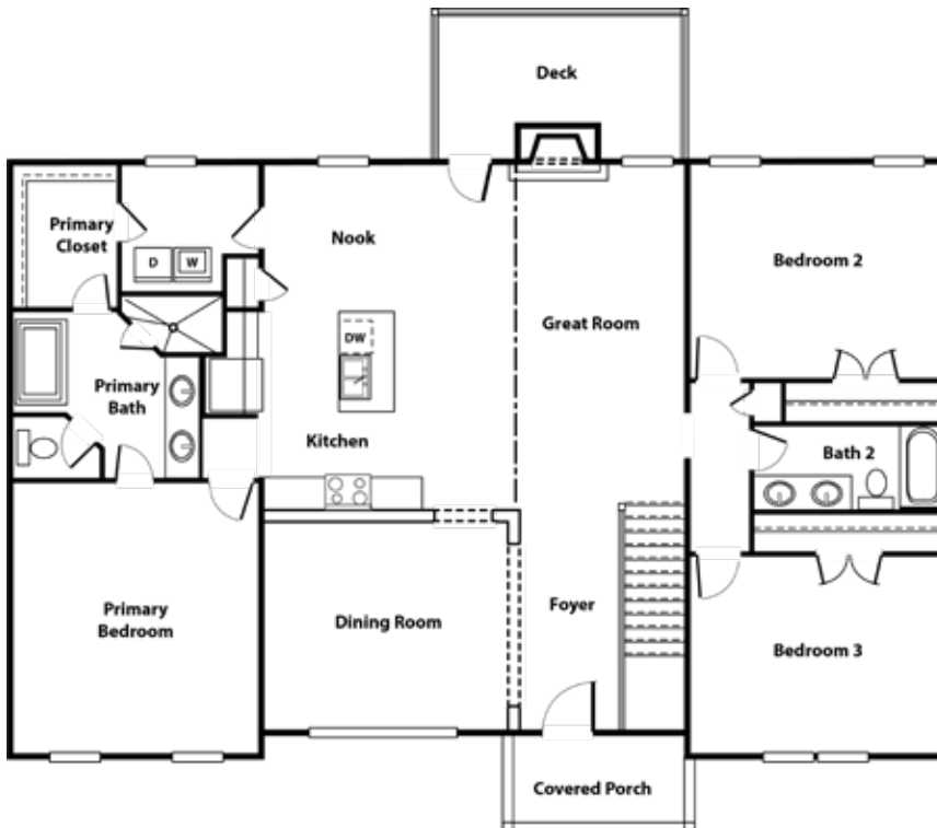
FIRST FLOOR
